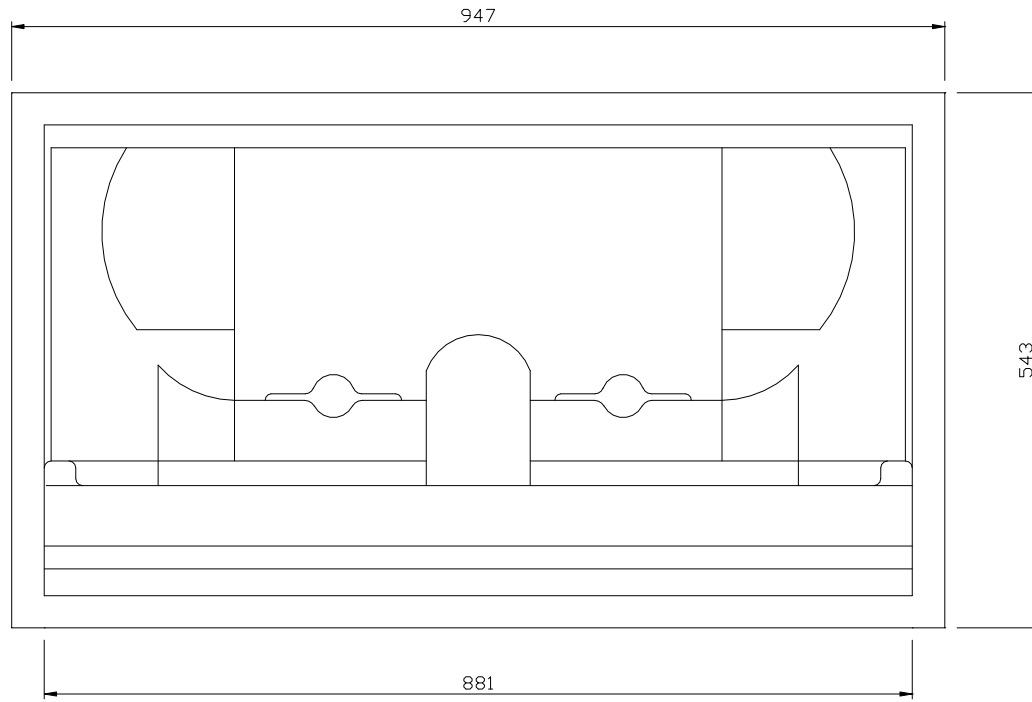
BELL-CHEM PRODUCTS COMPANY DOLPHIN CLAD STAINLESS STEEL NAPPY CHANGING UNIT RECESSED BC 100-SSC-R
